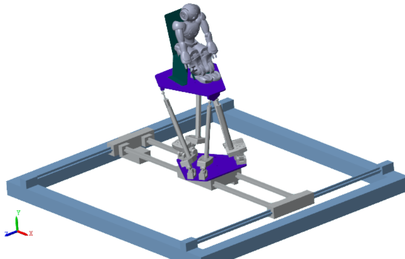
Figure 8.20 – Système multi-robot SimMechanics.
