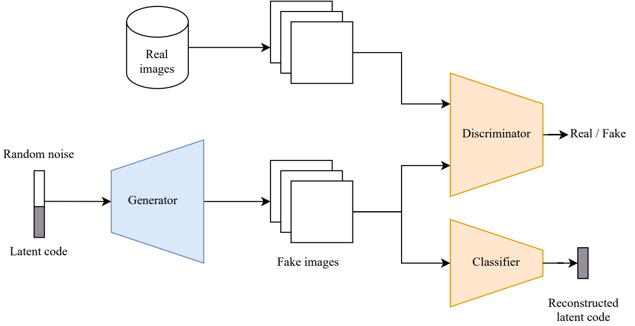
Figure 3.18: InfoGAN structure.
