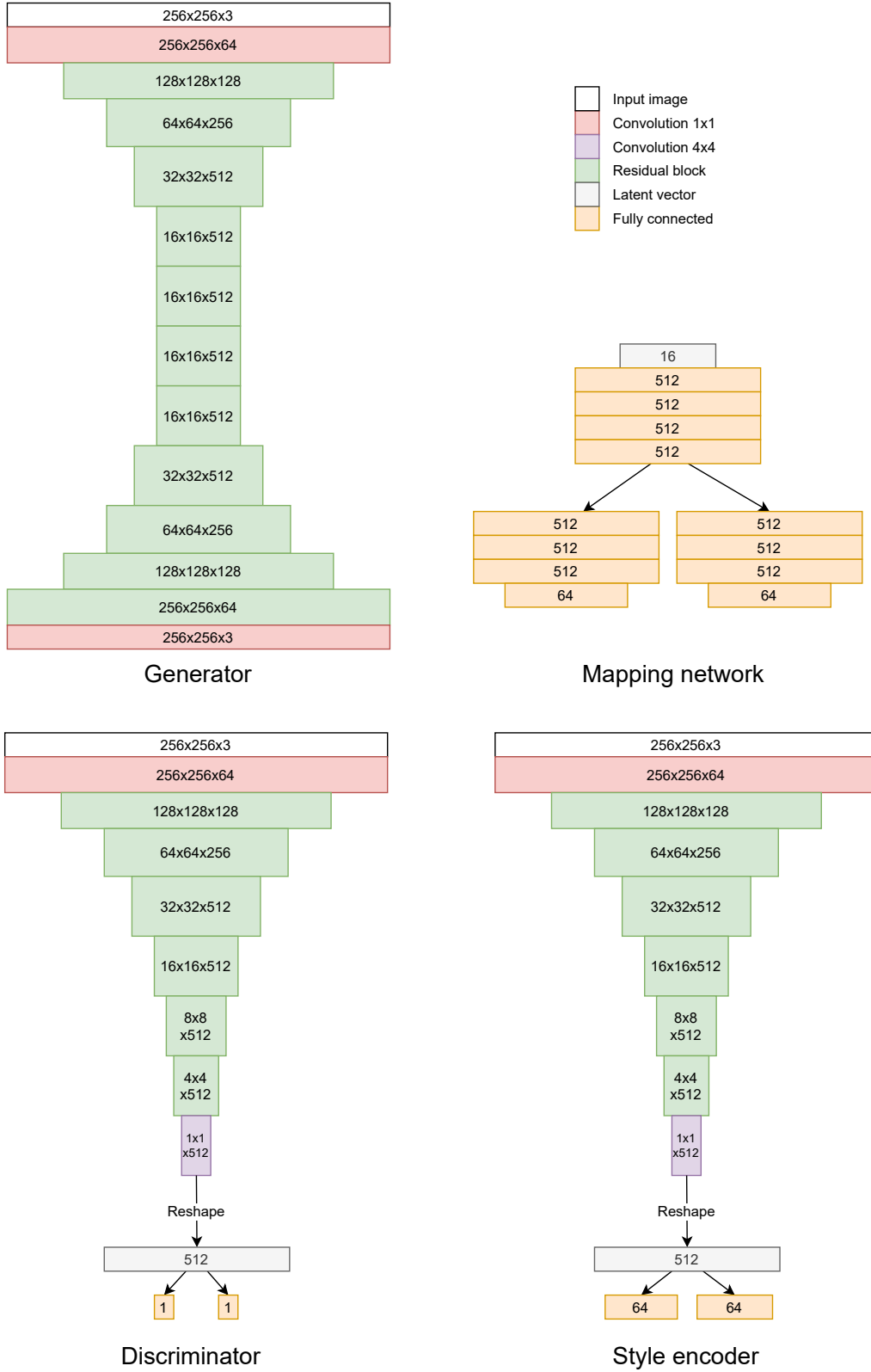
Figure 6.5: The architecture of each sub-network in StarGANv2: Generator (top-left), mapping-network (top-right), discriminator (bottom-left) and style encoder (bottom-right). In this example, the input image is in RGB with the size of 256 \times 256 .
