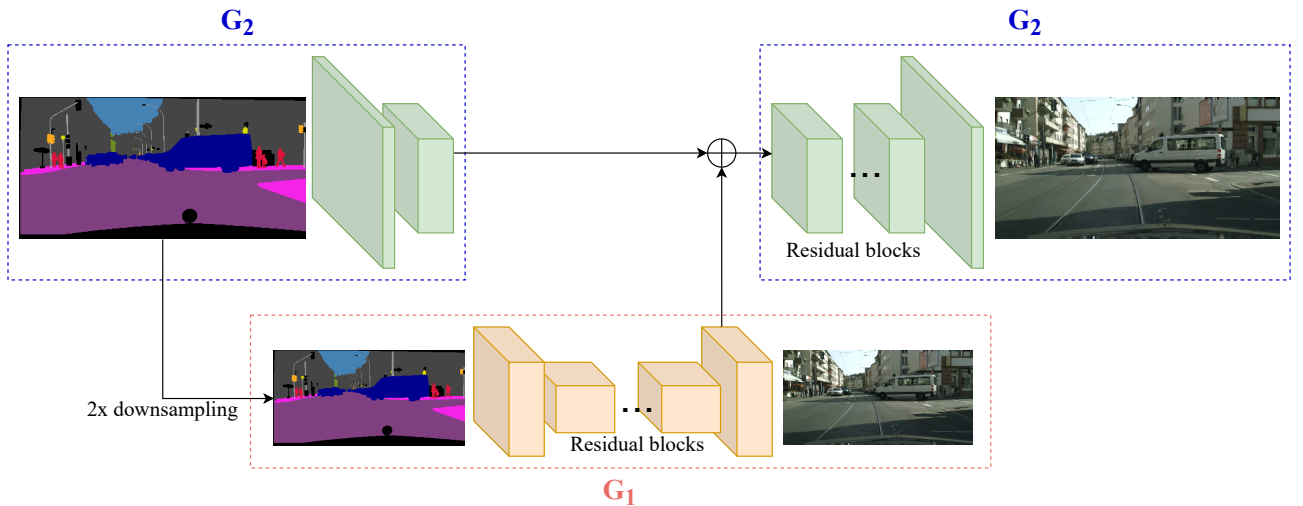
Figure 3.12: Pix2pixHD multi-resolution generator.
