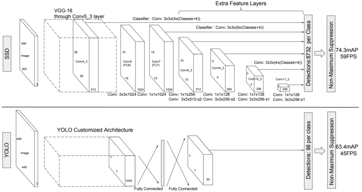
Figure 3.1: Comparison in the architecture of SSD and YOLO. Figure from [103]
