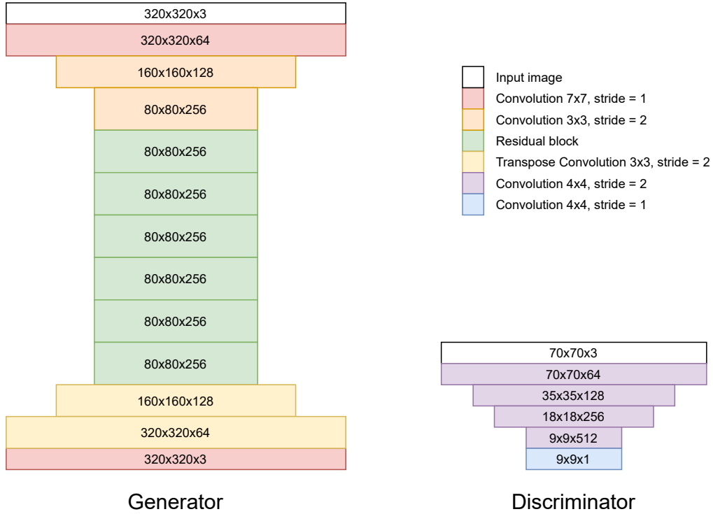
Figure 6.3: The architecture in details of the generators (left) and discriminators (right) in CycleGAN. For our experiment, the input image is in RGB with the size of 320x320.
