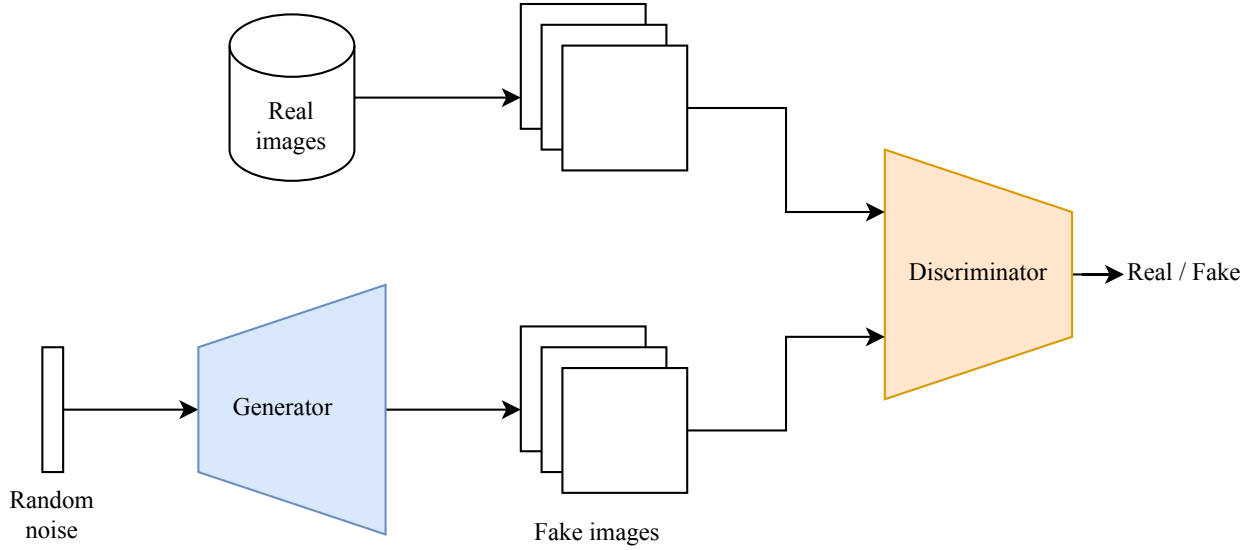
Figure 3.5: Generative adversarial network structure.
