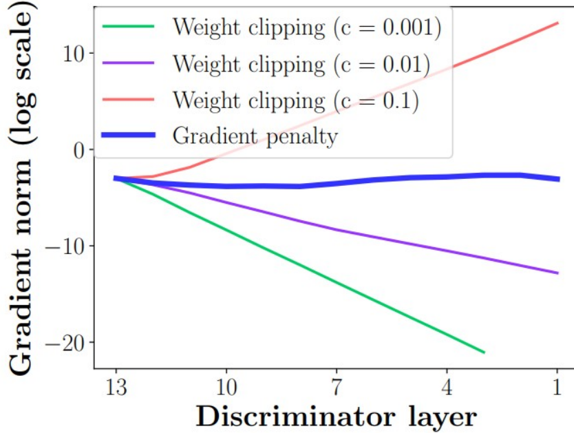
Figure 3.8: Gradient norms of WGAN critics (training on the Swiss Roll dataset [157]). A high value of c causes the gradient to explode, while its low value leads to the vanish of the gradient. The gradient is stable when a gradient penalty is applied. Figure from [59]
