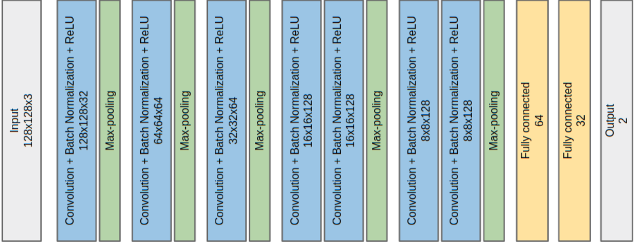
Figure 4.3: Gingivitis classifier architecture
