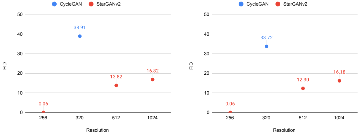
Figure 6.9: Comparison of the Fréchet Inception Distance (FID) between generated samples and real samples in the test set for the two methods CycleGAN and StarGANv2 (lower is better). The comparison is done on two tasks: generating aligner (left) and removing aligner (right).
