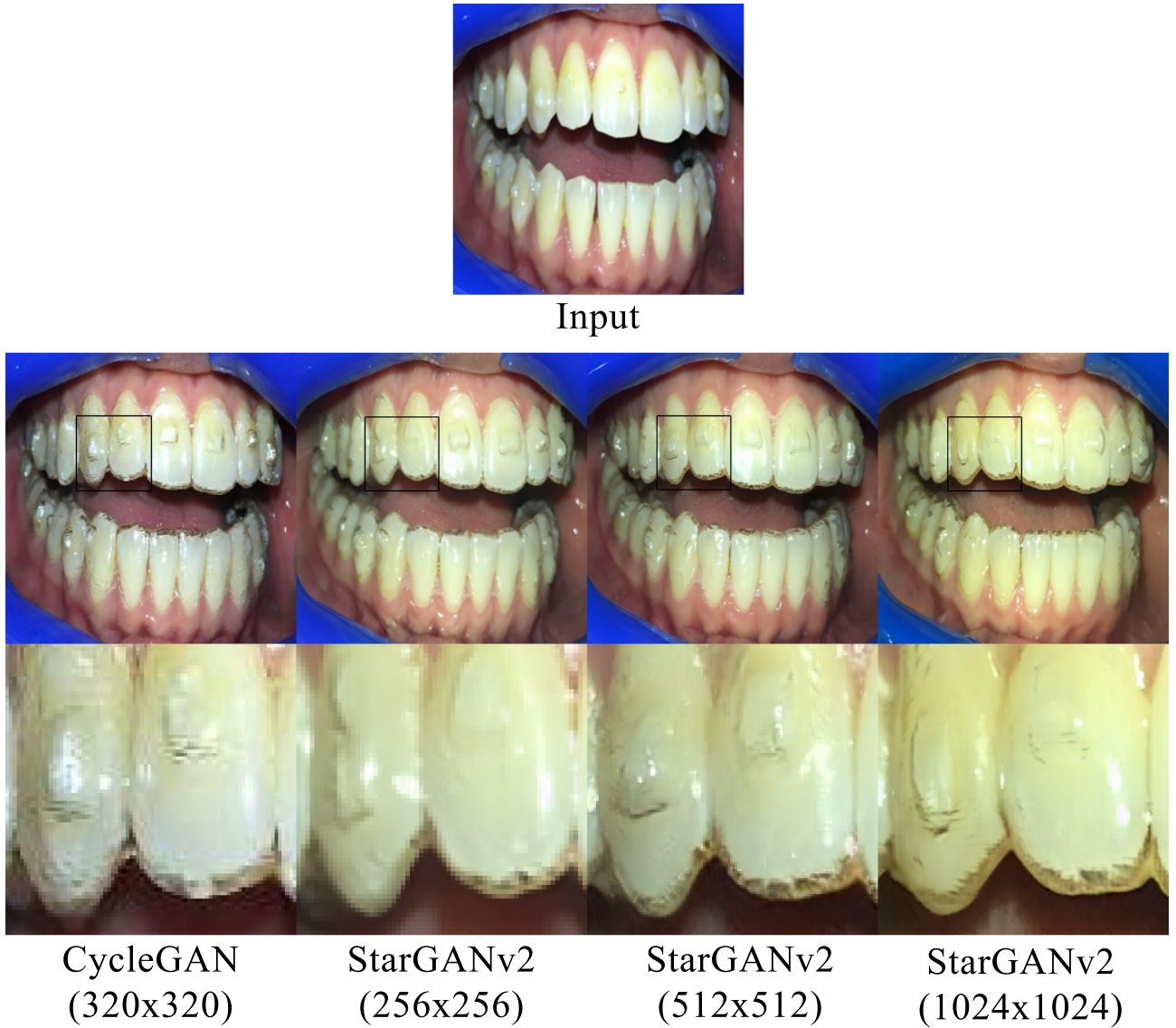
Figure 6.7: Qualitative comparison between outputs of CycleGAN and StarGANv2 at multiple resolutions for the task no-aligner→with-aligner.
