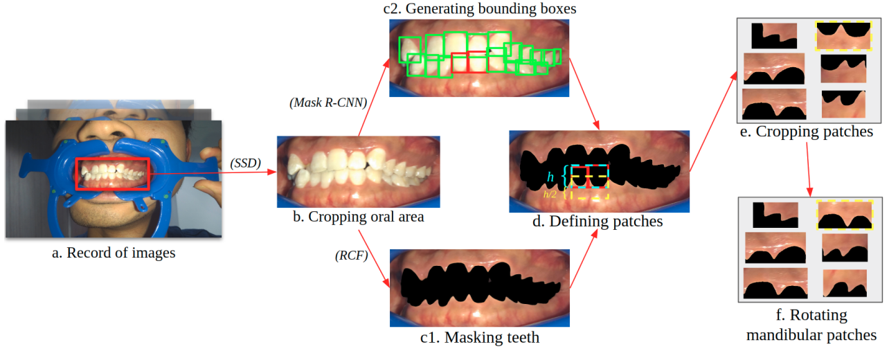
Figure 4.1: Preprocessing procedure
