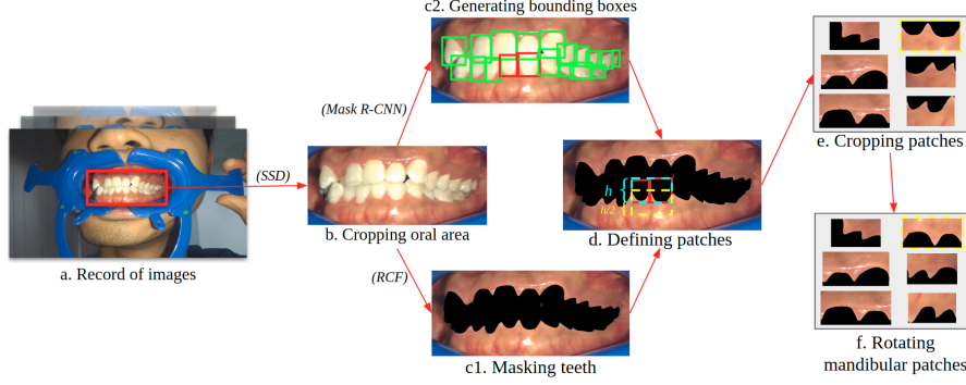
Fig. 1. Preprocessing procedure
