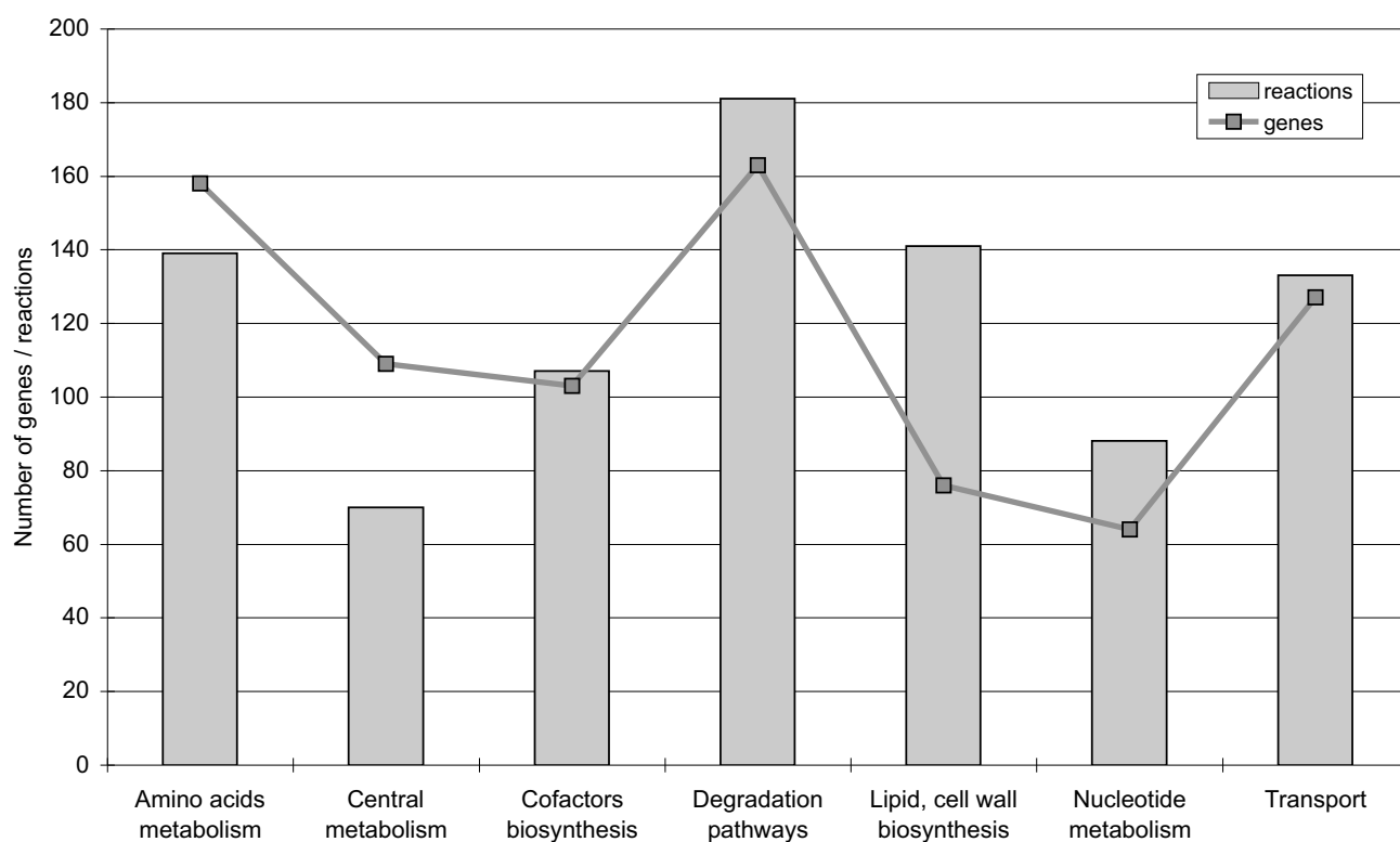
Figure 3 Number of reactions and genes in iAbayli v1 distributed by model metabolic categories. Reactions were associated with a unique metabolic category. Genes linked to several reactions may be associated with multiple categories.
