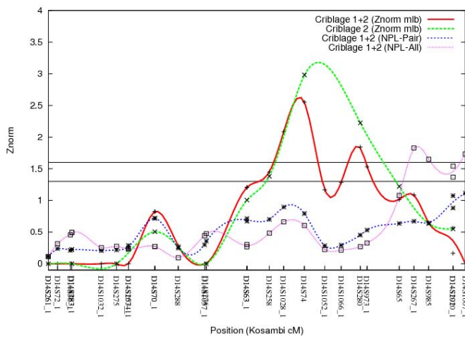
chromosome 14
