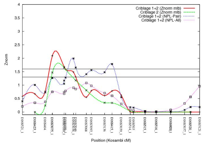
chromosome 16
